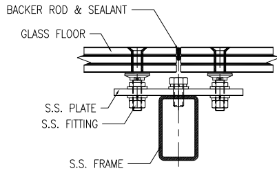
SECTION DETAIL EXTERIOR OR INTERIOR
