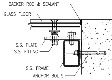
SECTION DETAIL @PERIPHERY
