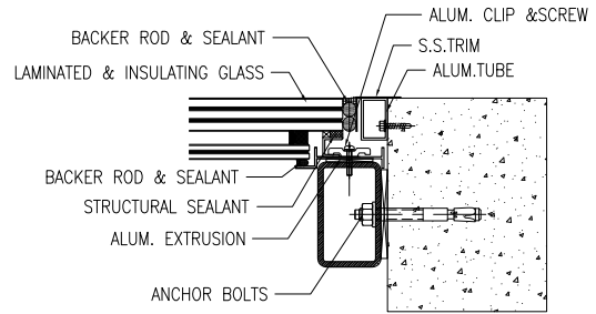
SECTION DETAIL EXTERIOR W/ THERMAL REQUIREMENT
