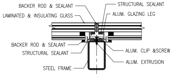
SECTION DETAIL EXTERIOR W/ THERMAL REQUIREMENT
