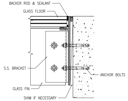
SECTION DETAIL @PERIPHERY
