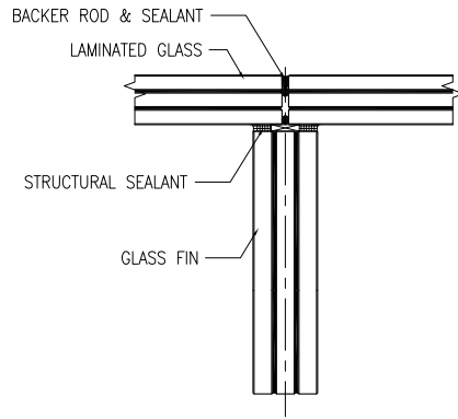
SECTION DETAIL EXTERIOR OR INTERIOR
