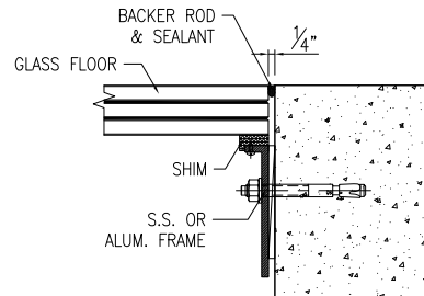
SECTION DETAIL @PERIPHERY
