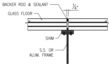
SECTION DETAIL ONLY FOR INTERIOR
