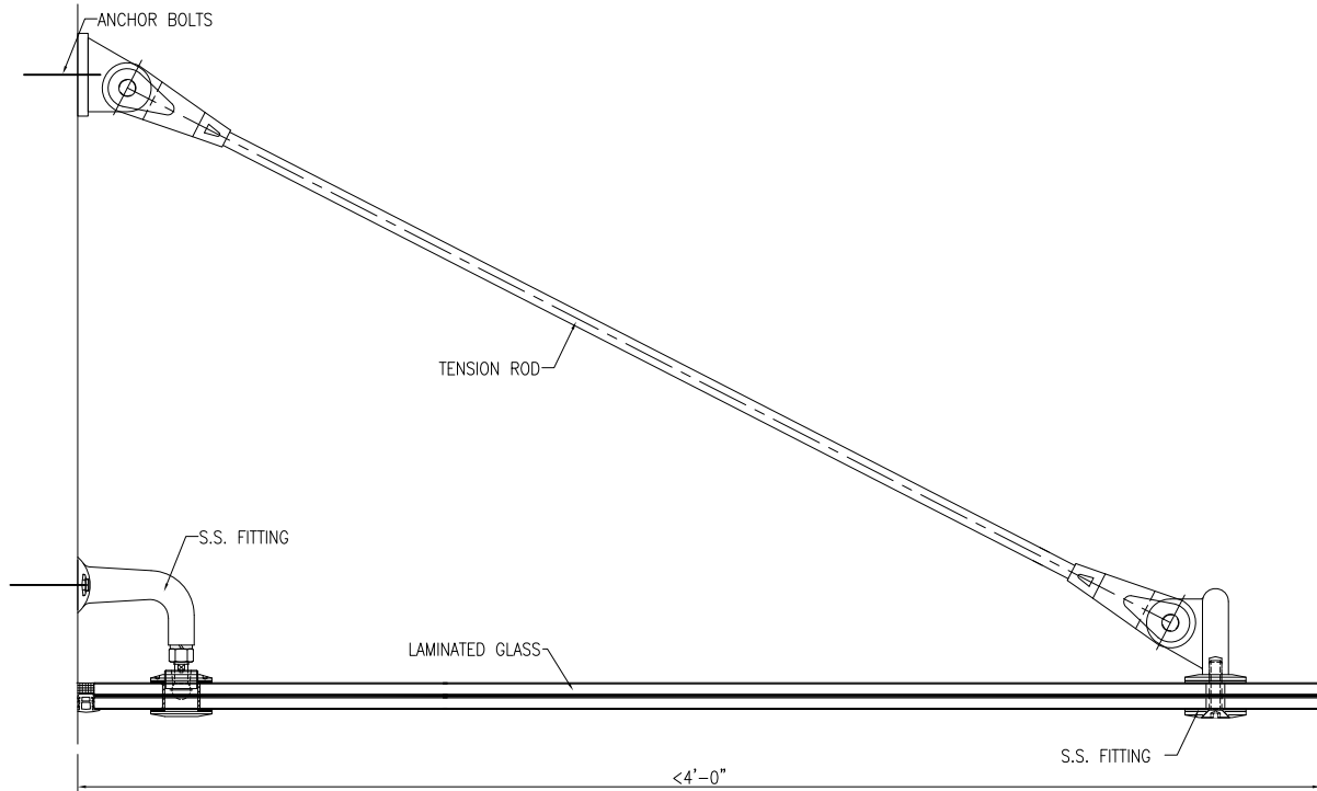
CANOPY SECTION
