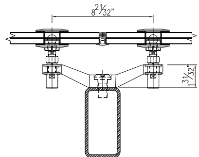
SECTION DETAIL TOP FIXING
