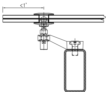
SECTION DETAIL TOP FIXING
