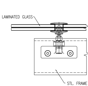
SECTION DETAIL SIDE FIXING
