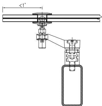
SECTION DETAIL TOP FIXING W/ CONNECTOR
