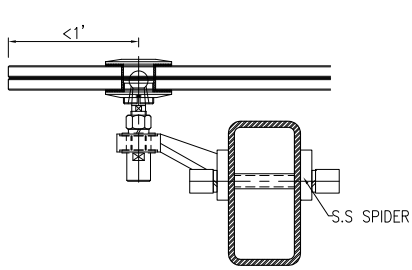
SECTION DETAIL SIDE FIXING
