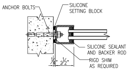
JAMB DETAIL S.S. CHANNEL
