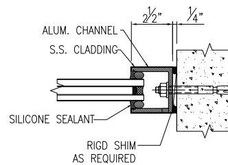
JAMB DETAIL ALUM. CHANNEL
