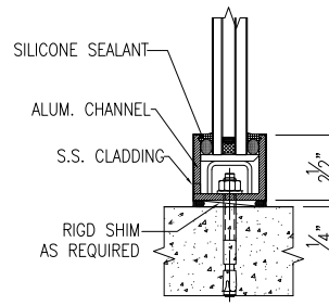
SILL DETAIL
