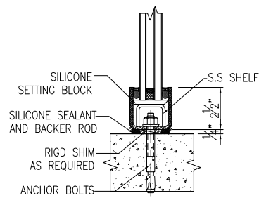
SILL DETAIL
