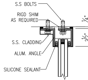
HEAD DETAIL
