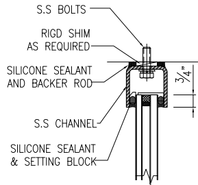
HEAD DETAIL
