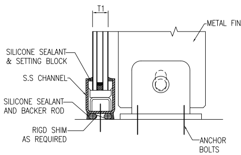
SILL DETAIL
