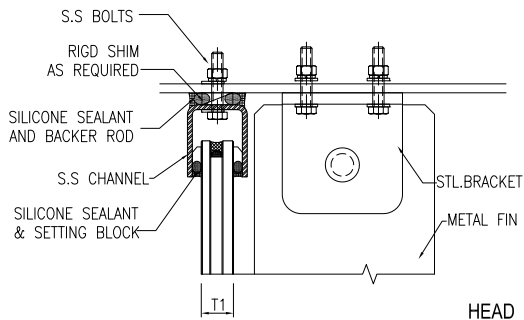
HEAD DETAIL
