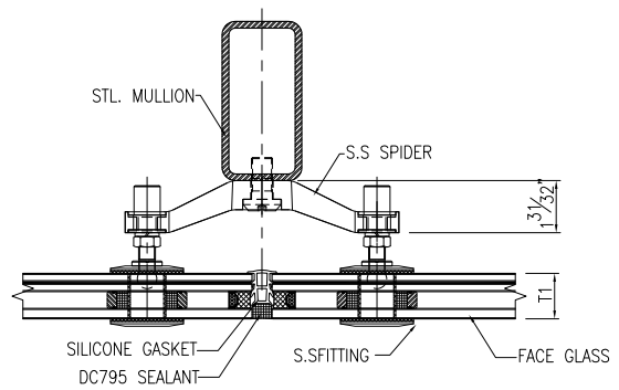
PLAN DETAIL FRONT FIXING SPIDER FITTING
