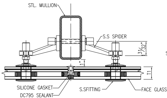
PLAN DETAIL SIDE FIXING SPIDER FITTING
