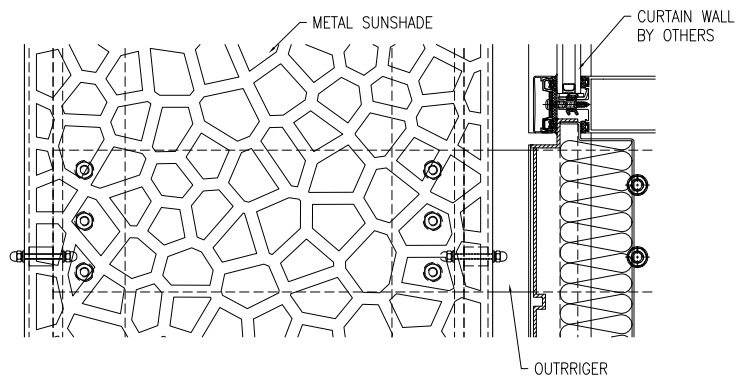
TYPICAL SECTION DETAIL
