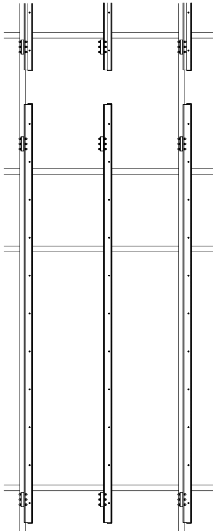
PARTIAL ELEVATION
