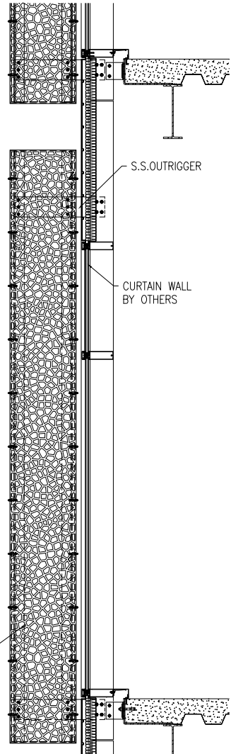
TYPICAL SECTION
