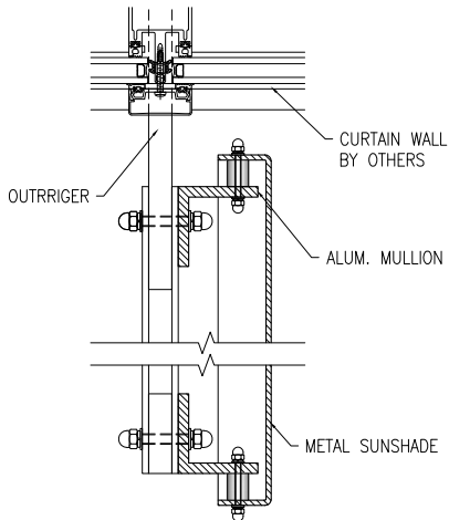
TYPICAL PLAN DETAIL
