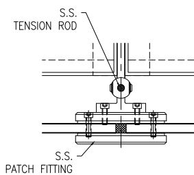
TYPICAL PLAN DETAIL
