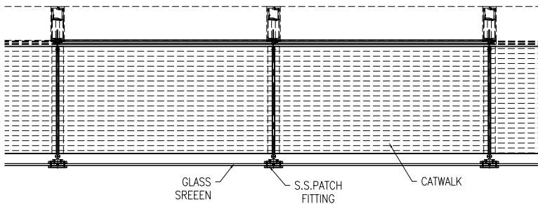
TYPICAL PLAN
