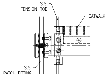
TYPICAL SECTION DETAIL
