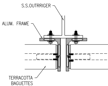
TYPICAL PLAN DETAIL
