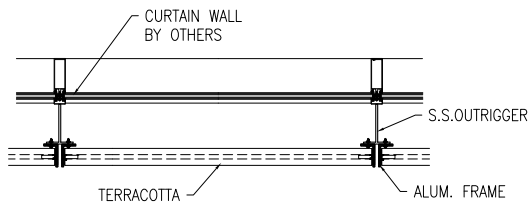
TYPICAL PLAN
