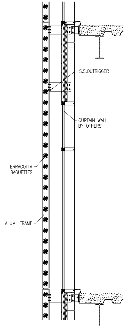
TYPICAL SECTION
