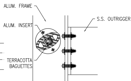
TYPICAL SECTION DETAIL
