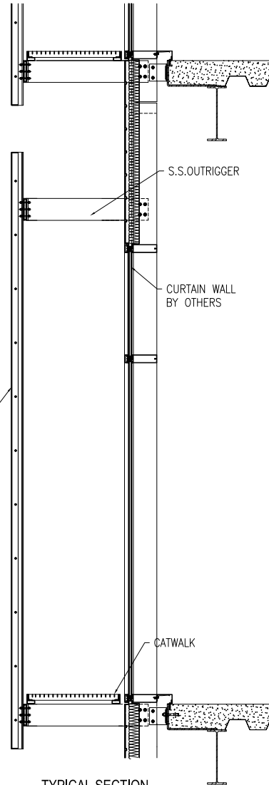
TYPICAL SECTION
